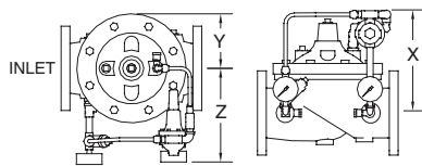
Globe Pilot System Dimensions
