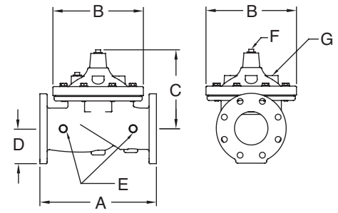
Globe Style Body
