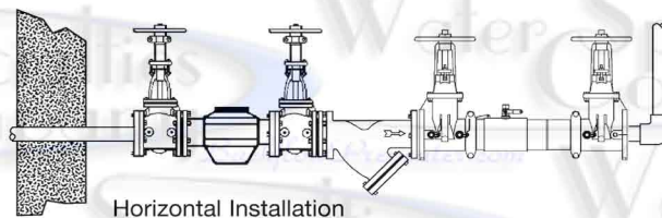
Horizontal Installation
