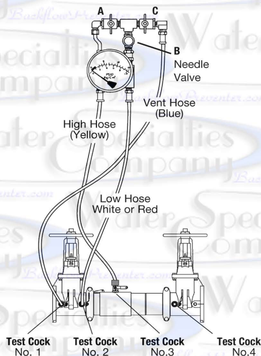
Ball Type Test Valves
