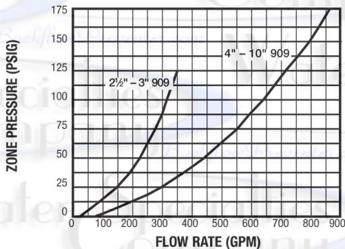
Figure 1 Series 909 RELIEF VALVE DISCHARGE RATES
