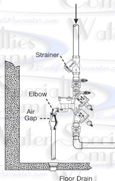
Watts 1/4" – 2" 919 *Vertical Flow Down
