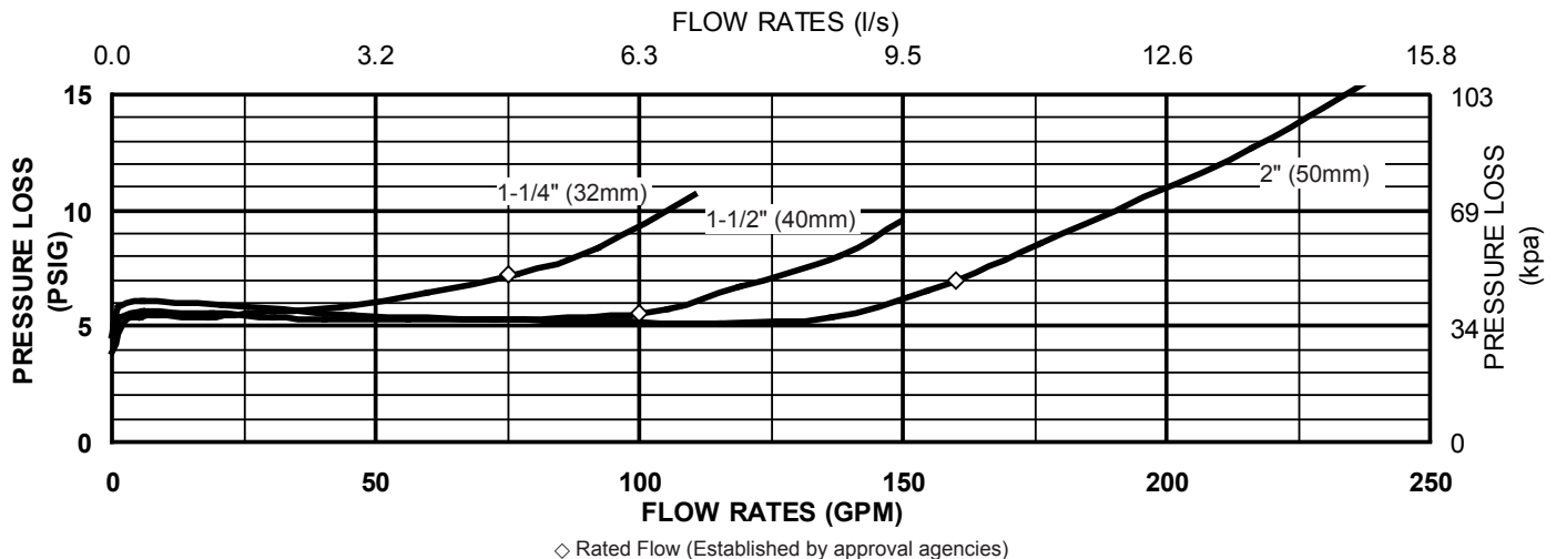
Capacity thru Schedule 40 Pipe
