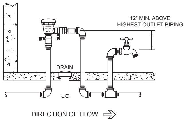
INDOOR INSTALLATION
